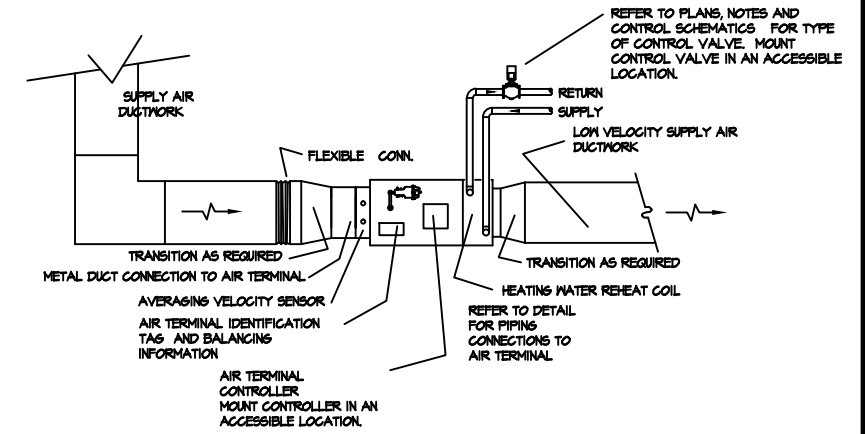
⑤ TYPICAL AIR TERMINAL DETAIL FIRST AND 2ND FL SOILED PROCESSING
