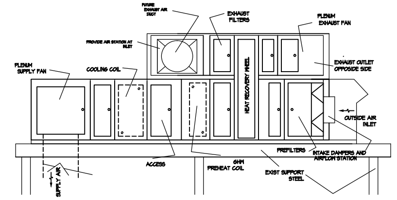
③ ELEVATION AT AHU-1
