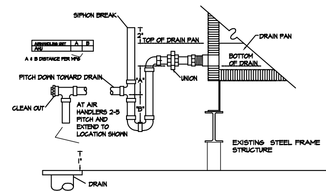
⑥ CONDENSATE DRAIN PIPING DETAIL
