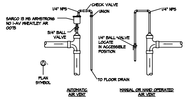
⑦ AIR ELIMINATOR DETAIL
