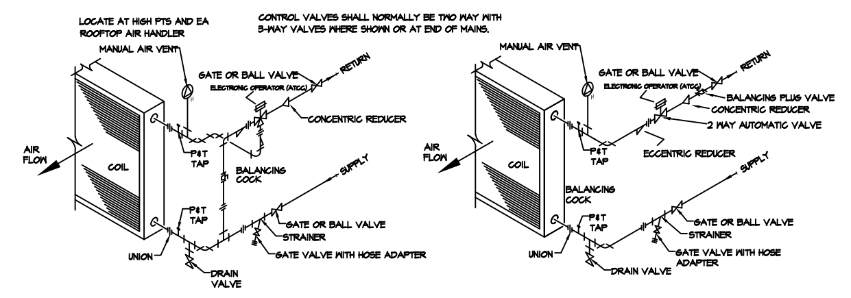
⑧ WATER COIL PIPING W/ TWO AND THREE WAY VALVES
