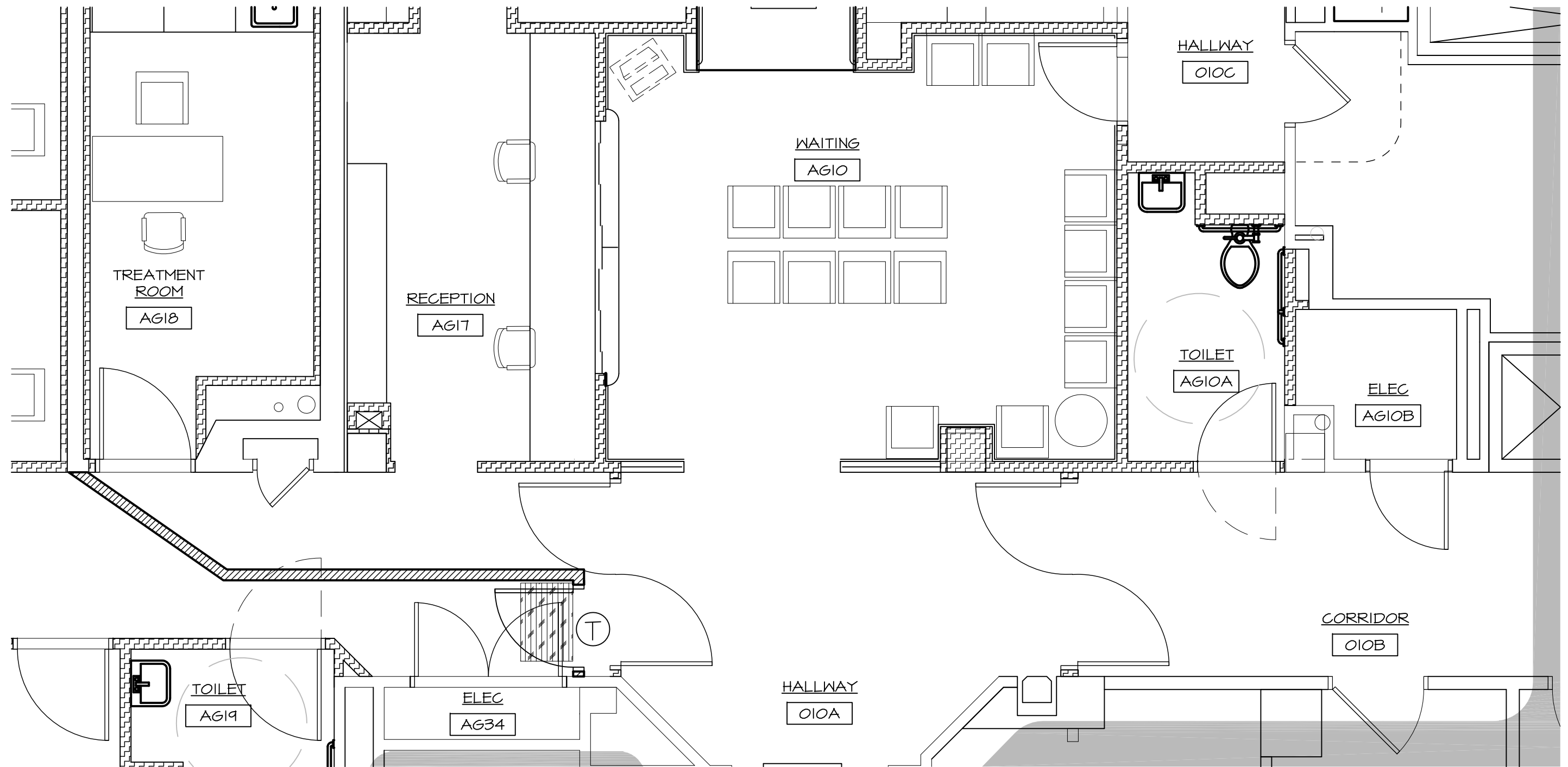
1 GROUND FLOOR PHASING FLOOR PLAN PHASE 2 1/4"
