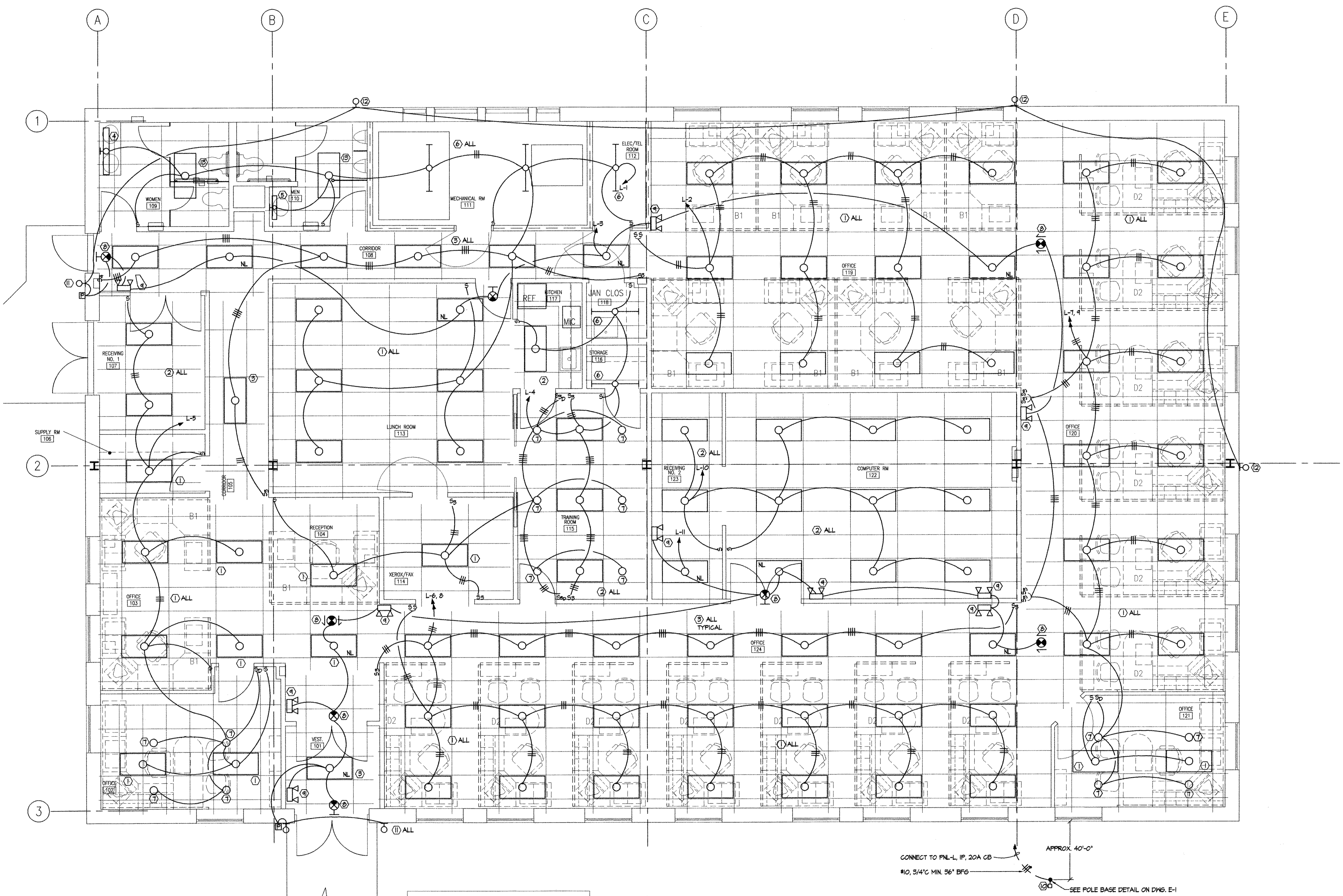
1 FLOOR PLAN - LIGHTING E2 SCALE: 1/4" = 1'-0"
