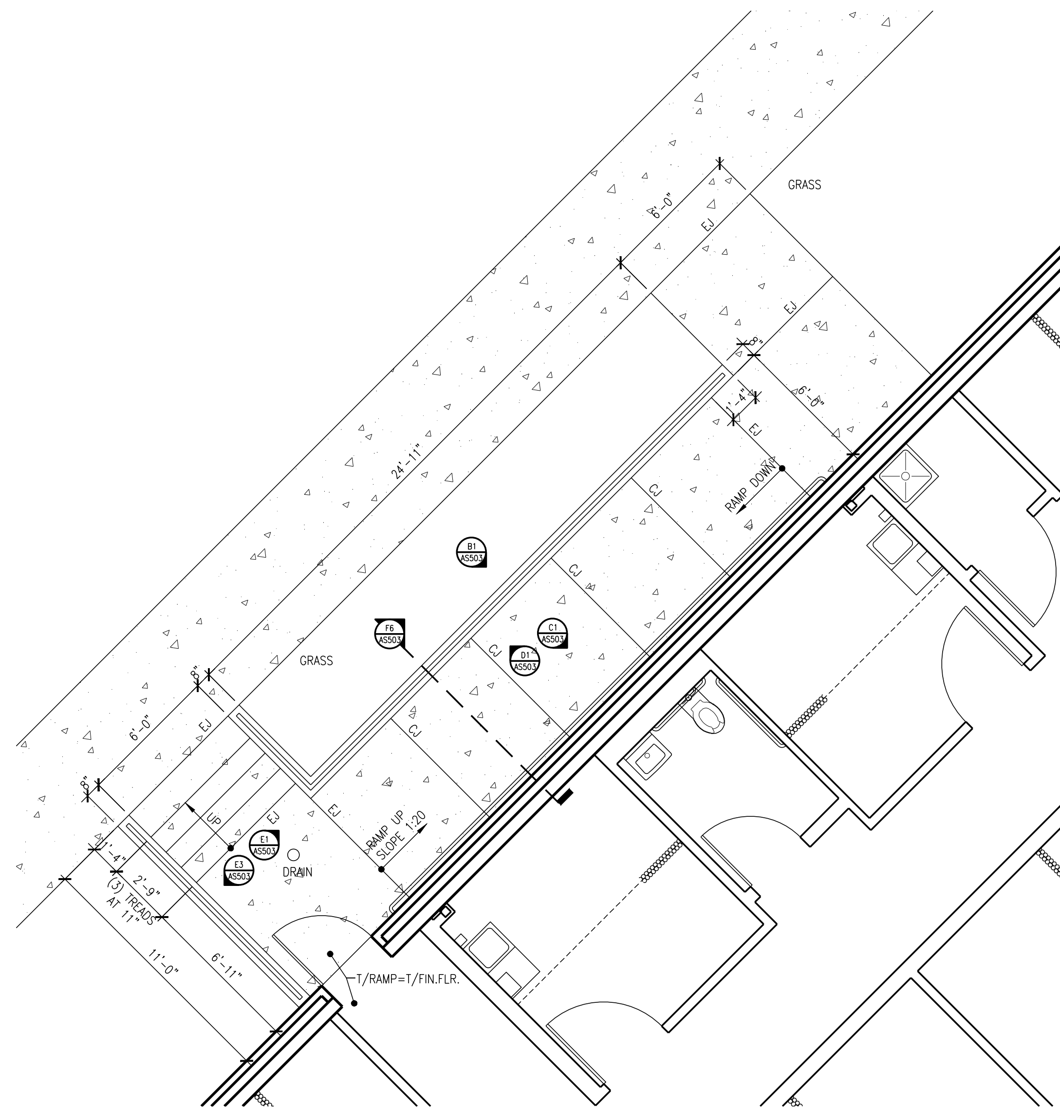
C3 ENLARGED PLAN, NORTH EXTERIOR RAMP AND STAIRS 1/4"=1'-0"
