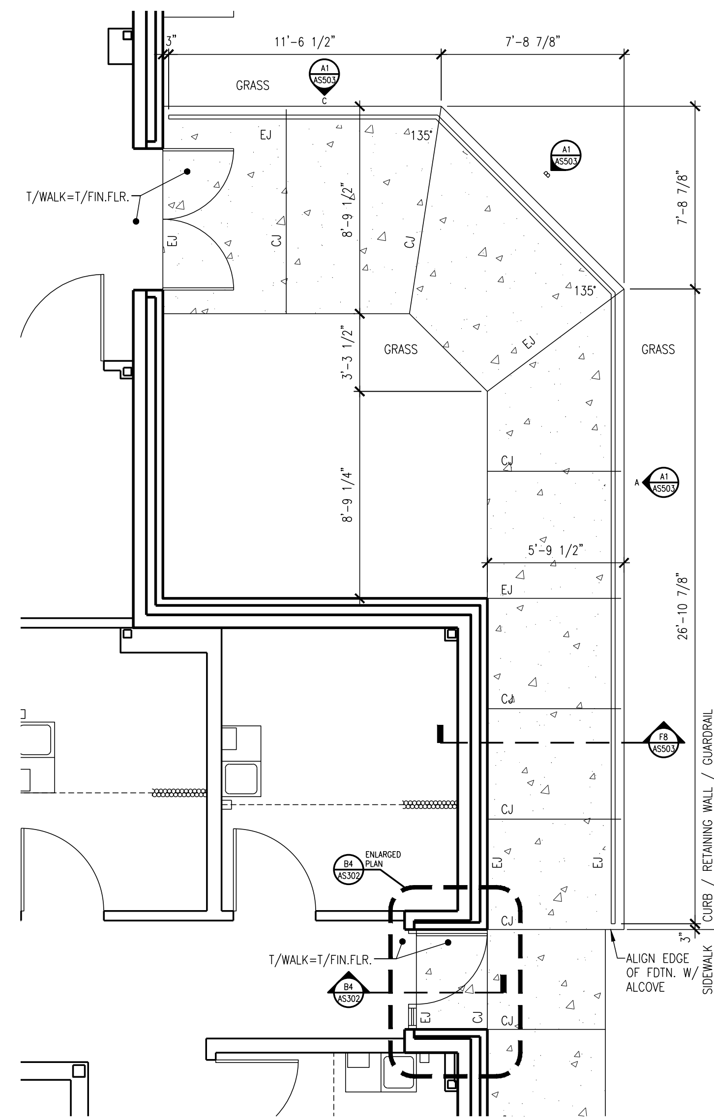
C6 ENLARGED PLAN, SOUTH EXTERIOR 1/4"=1'-0"
