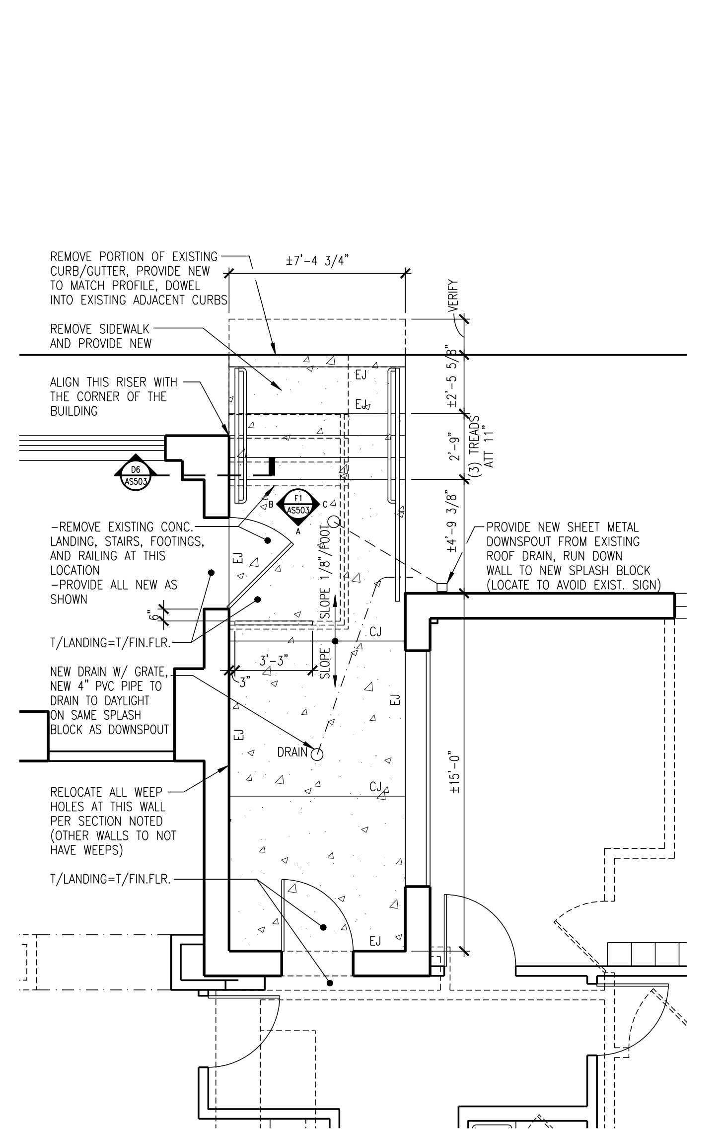
C8 ENLARGED PLAN, EAST EXTERIOR 1/4"=1'-0"
