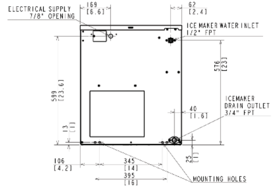
AIR-COOLED UNIT
