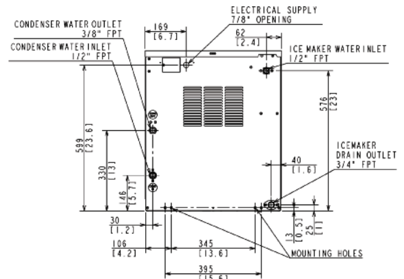
WATER-COOLED UNIT
