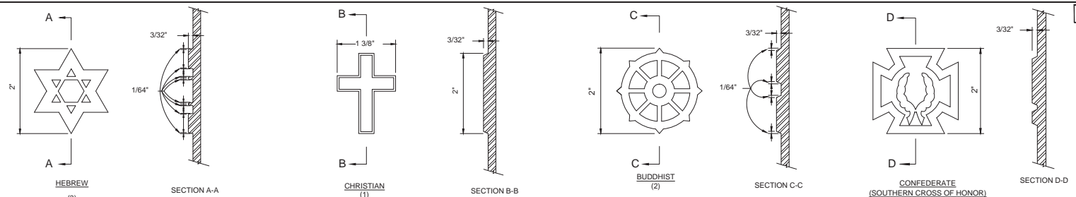
RAISED BRONZE SCALE: 1"=1"
