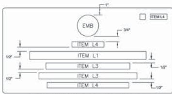
5 LINE INSCRIPTION PLACEMENT AND DETAIL
