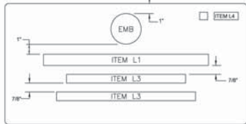
3 LINE INSCRIPTION PLACEMENT AND DETAIL
