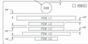
5 LINE INSCRIPTION PLACEMENT AND DETAIL
