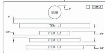
4 LINE INSCRIPTION PLACEMENT AND DETAIL
