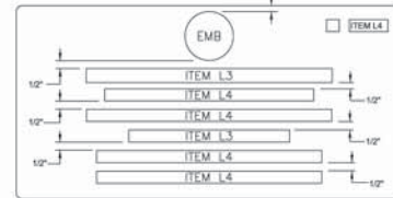
6 LINE INSCRIPTION PLACEMENT AND DETAIL
