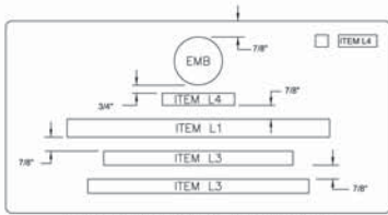
4 LINE INSCRIPTION PLACEMENT AND DETAIL
