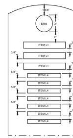
7 LINE INSCRIPTION PLACEMENT AND DETAIL
