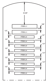
11 LINE INSCRIPTION PLACEMENT AND DETAIL
