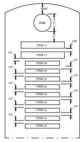
9 LINE INSCRIPTION PLACEMENT AND DETAIL
