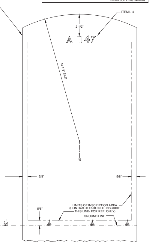
REAR FACE OF STONE SHOWING CORRECT LOCATION OF SECTION & GRAVE NUMBER (SEE DWG. A-W1-2 FOR REVERSE INSCRIPTION LOCATION if required)
