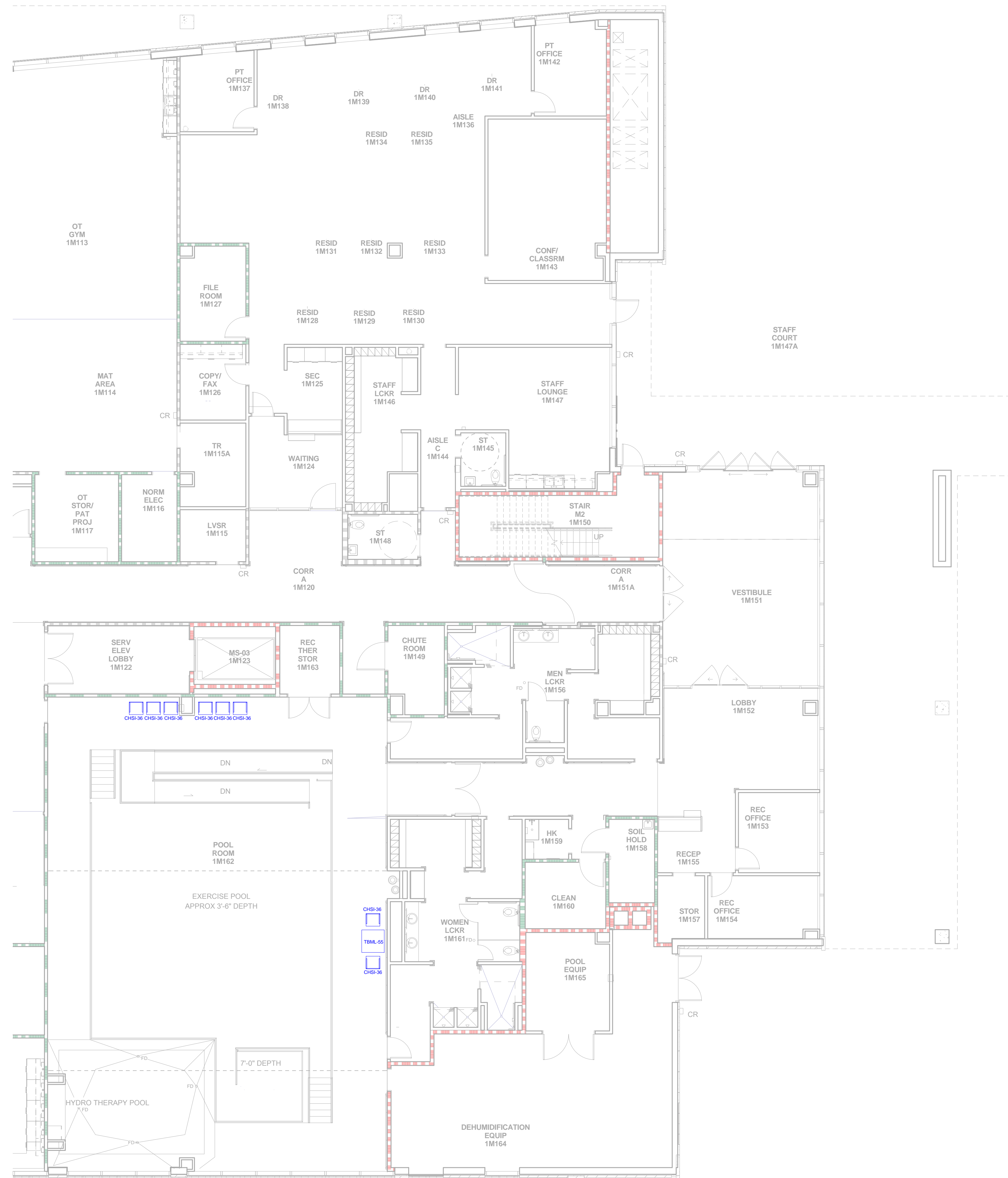
1 1st Floor Furniture Plan - Area M2 1/8" = 1'-0"
