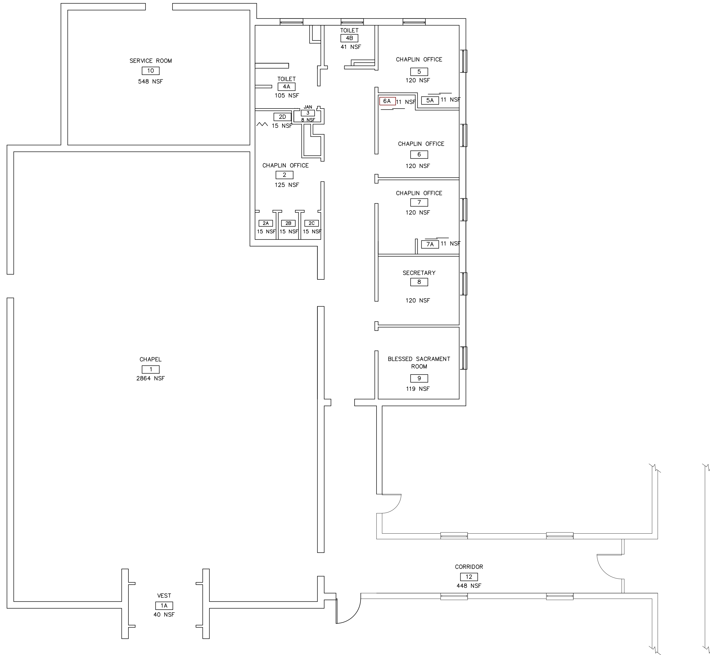
BUILDING 106 FIRST FLOOR PLAN SCALE: NONE
