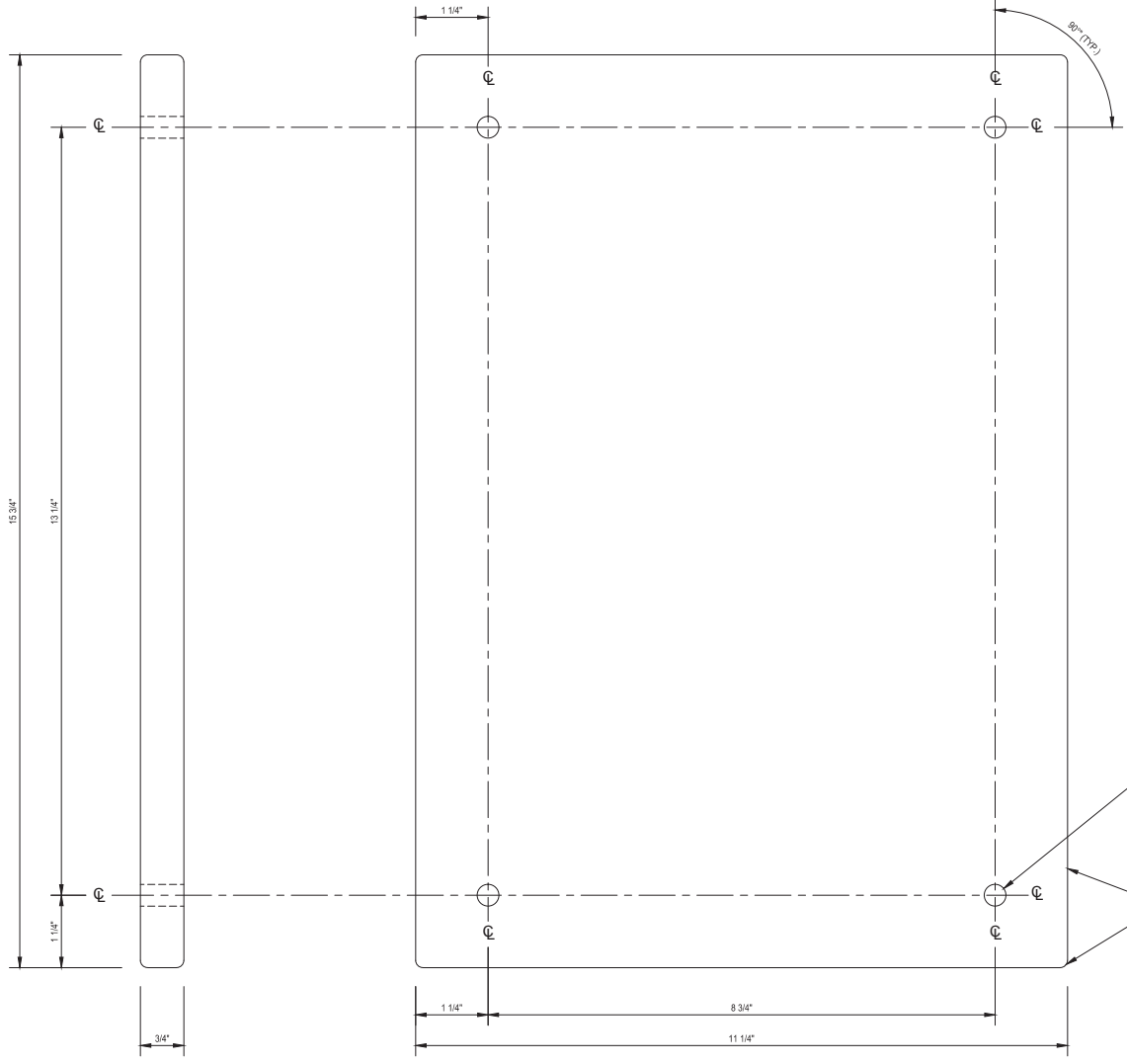
SIDE VIEW
