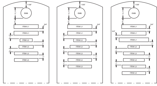
6 LINE INSCRIPTION PLACEMENT AND DETAIL
