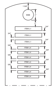
10 LINE INSCRIPTION PLACEMENT AND DETAIL
