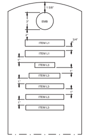
7 LINE INSCRIPTION PLACEMENT AND DETAIL
