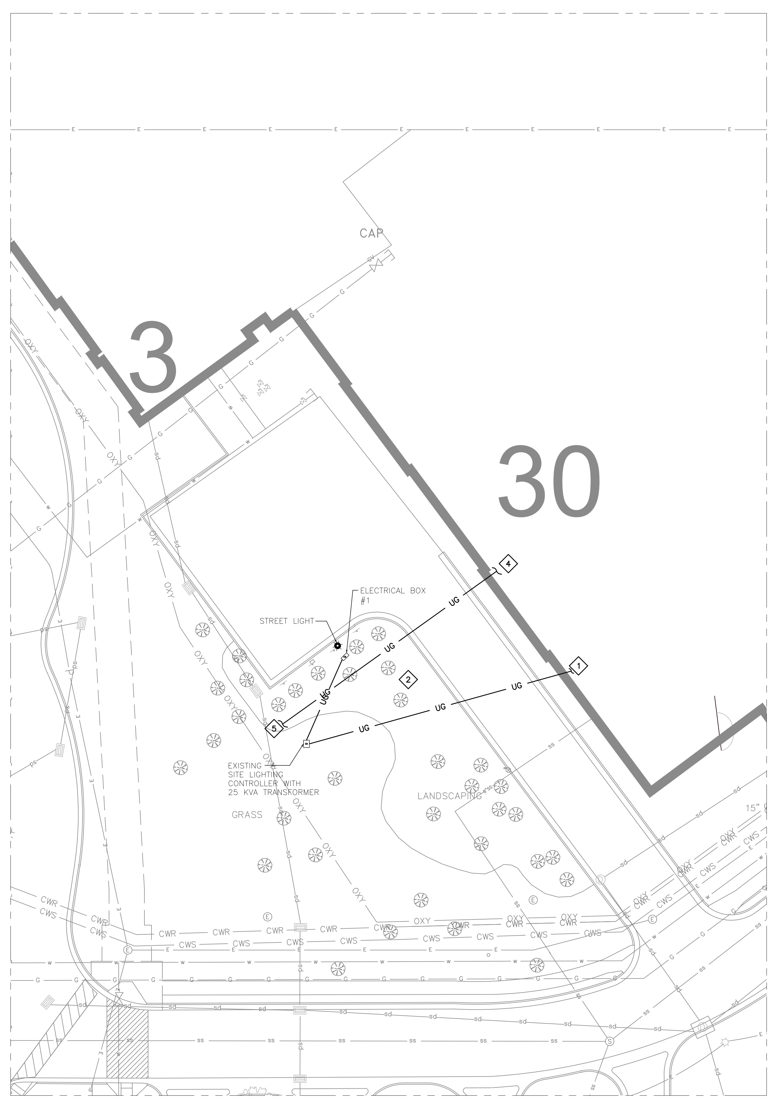
1 ELECTRICAL SITE PLAN-EXISTING E-200[E-200] 1" = 20'
