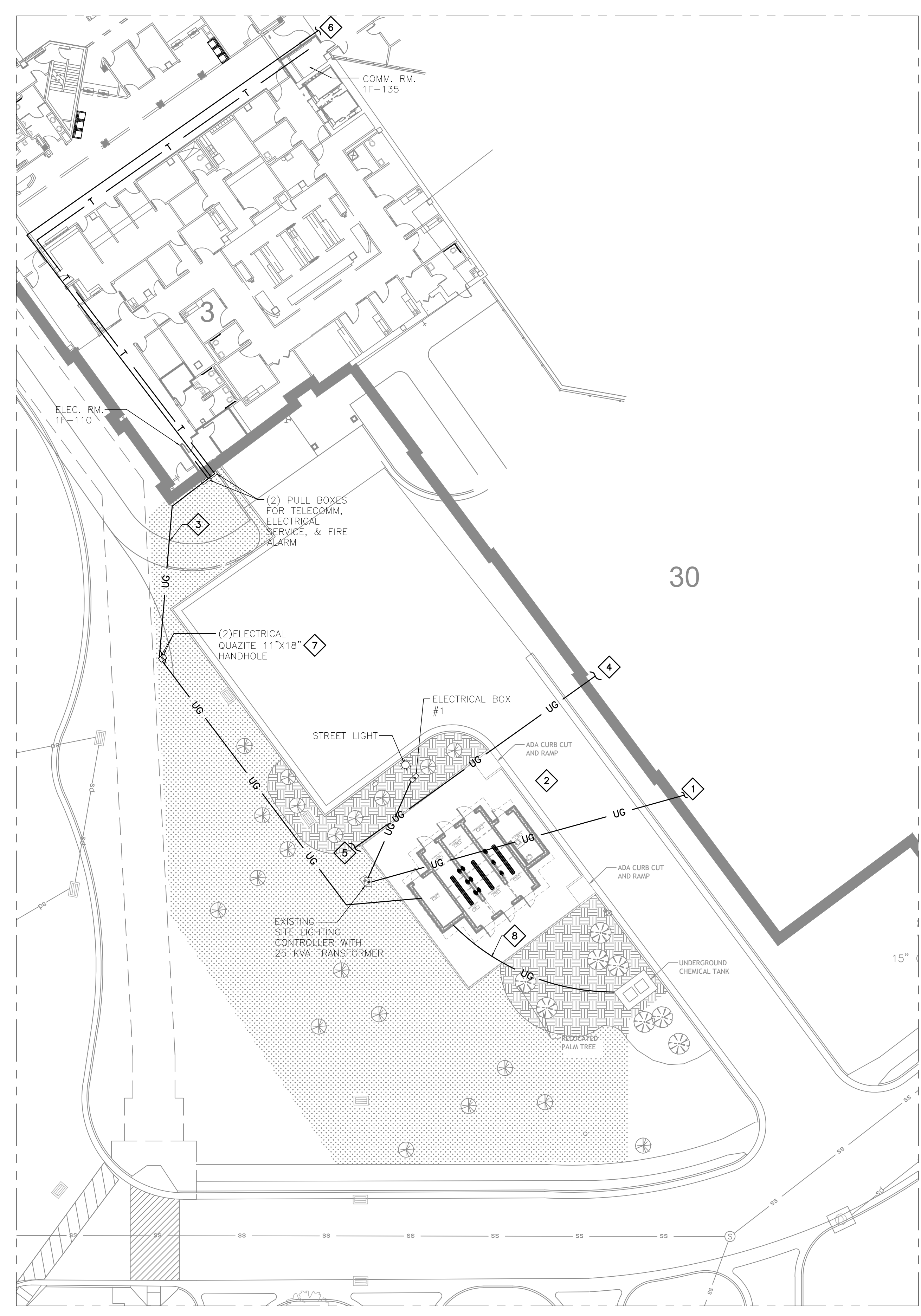
2 ELECTRICAL SITE PLAN-PHASE 1 INSTALL E-200[E-200] 1" = 20'
