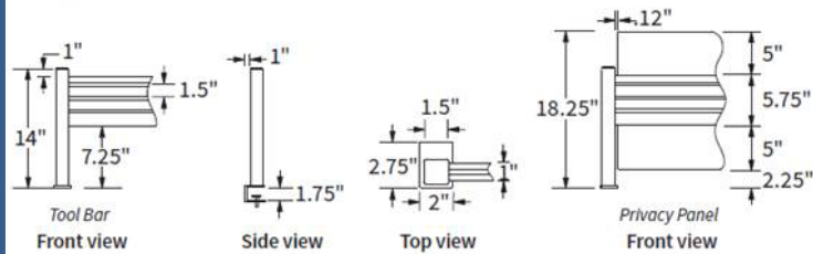
Tool Bar & Privacy Panel Component Dimensions
