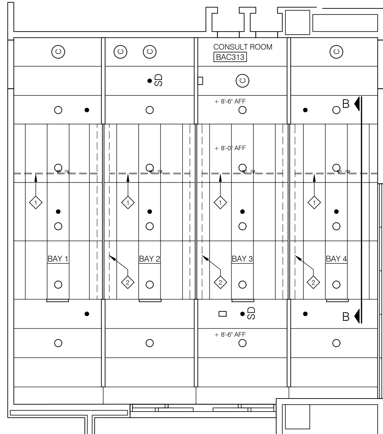
2 Pharmacy BAC313 Reflected Ceiling Plan Scale: 1/4" = 1'-0" 1-01
