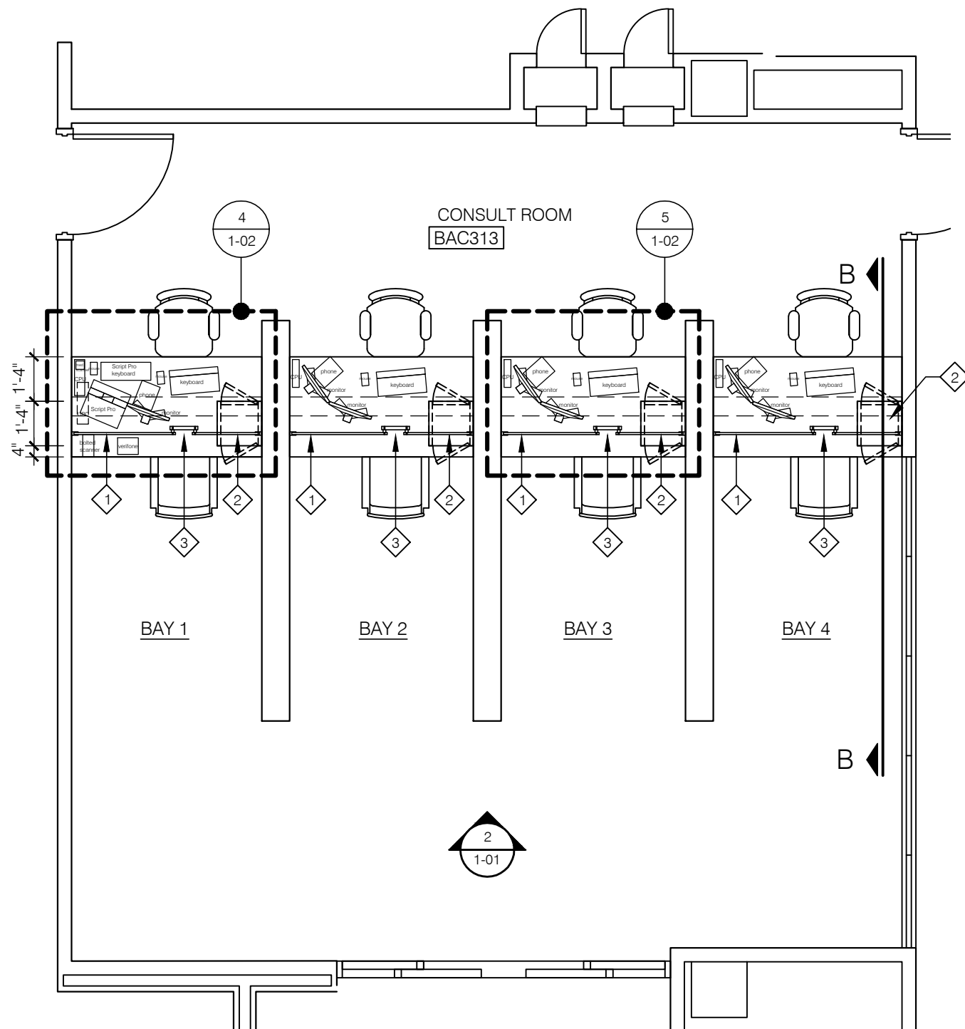
1 Pharmacy BAC313 Floor Plan Scale: 1/4" = 1'-0" 1-01
