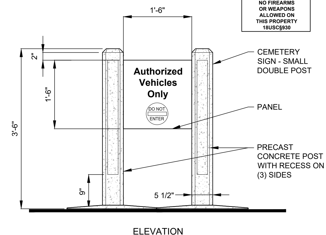
F8 SMALL DOUBLE POST SIGN LS101 1"=1'-0"
