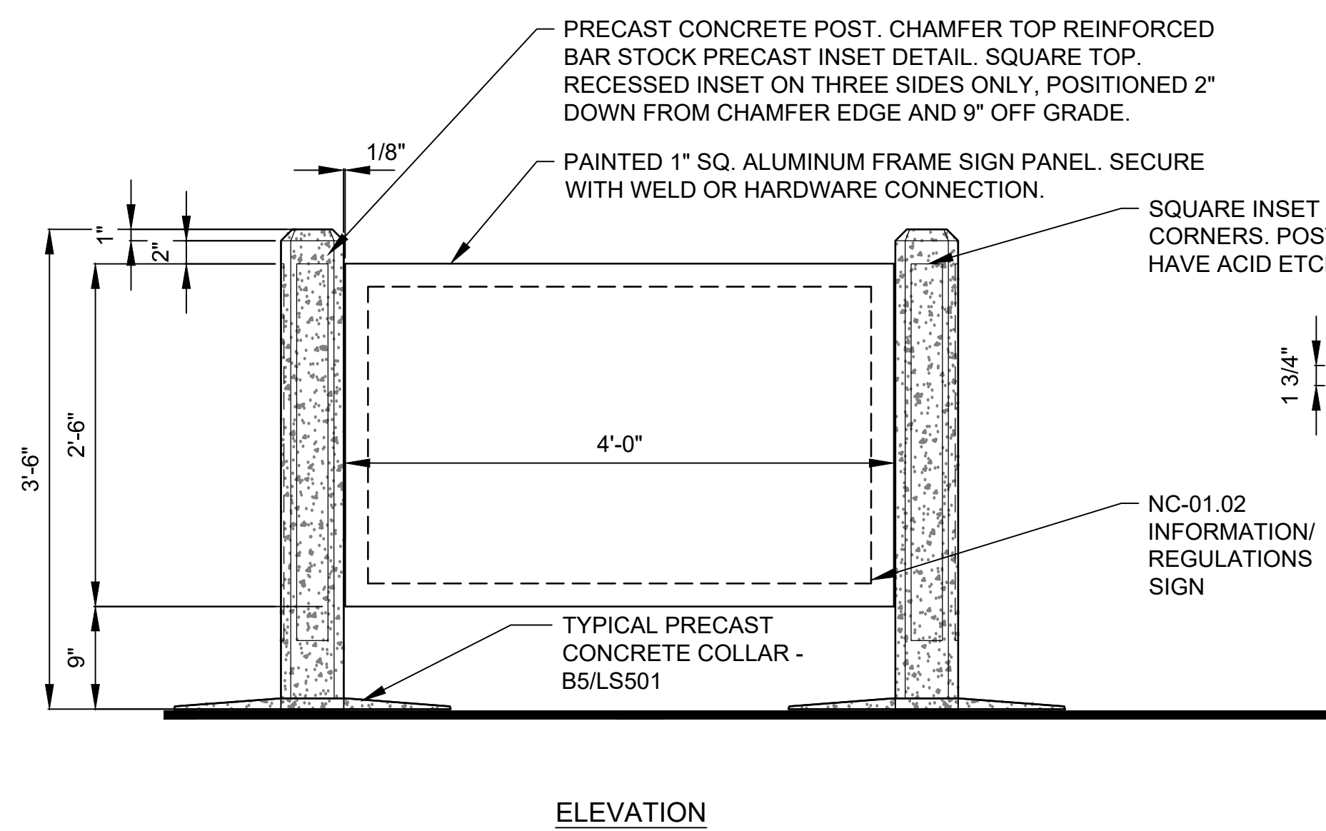
F3 PRECAST CONCRETE DOUBLE POST AND PANEL LS501 NOT TO SCALE
