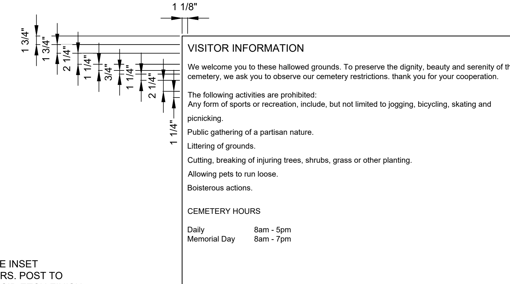
C5 WALL MOUNTING: NON-ILLUMINATED SIGNS LS103 1"=1'-0"
