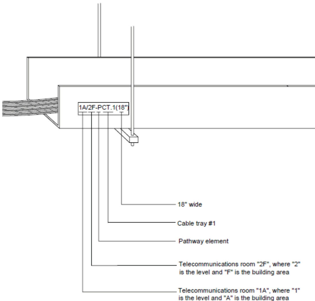
Pathway Label (cable tray)
