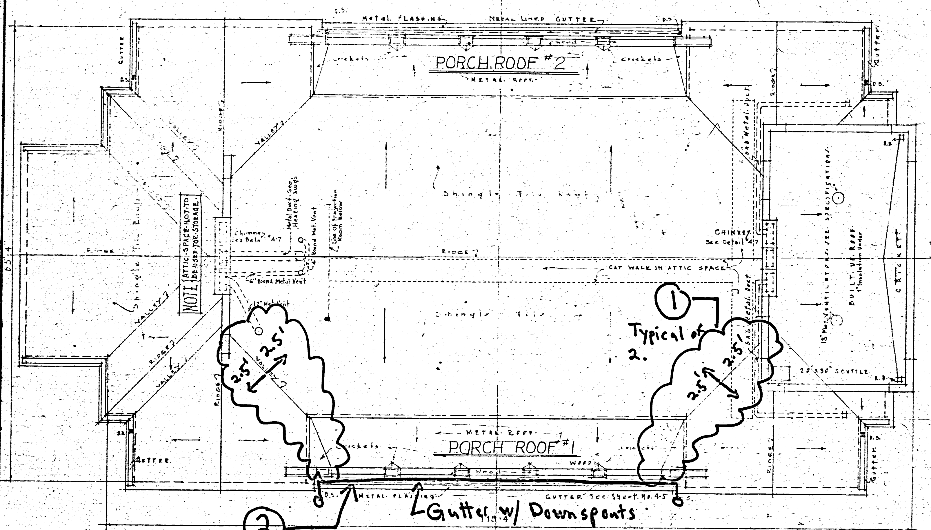
ROOF PLAN SCALE - 1/8" = 1'-0"
