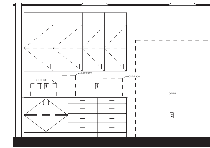
9 LAB Elevation A002-9 1/2" = 1'-0"
