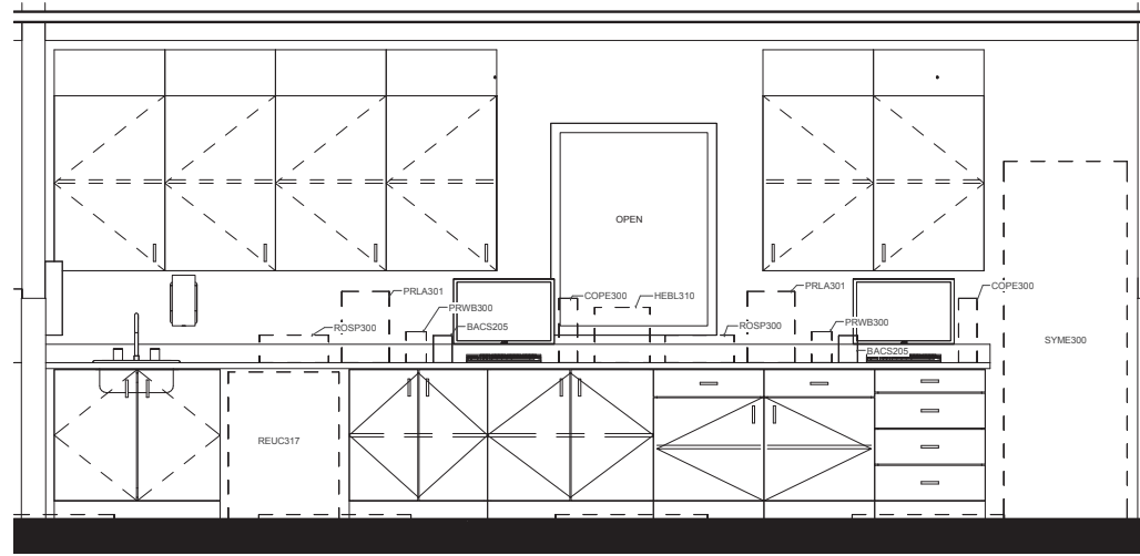
1 LAB Elevation A002-1 1/2" = 1'-0"
