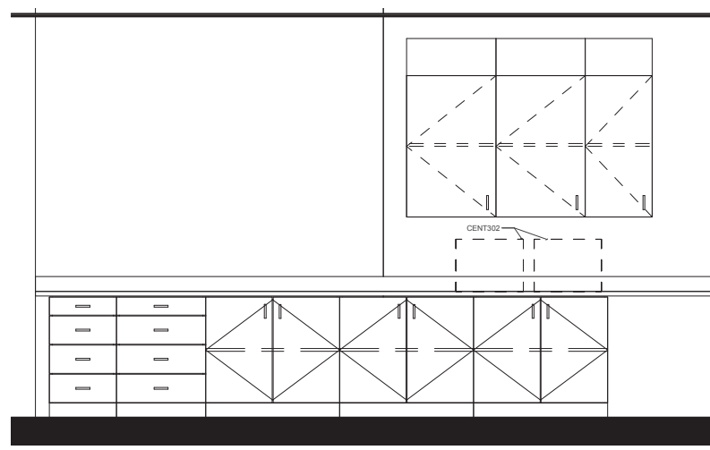
3 LAB Elevation A002-3 1/2" = 1'-0"
