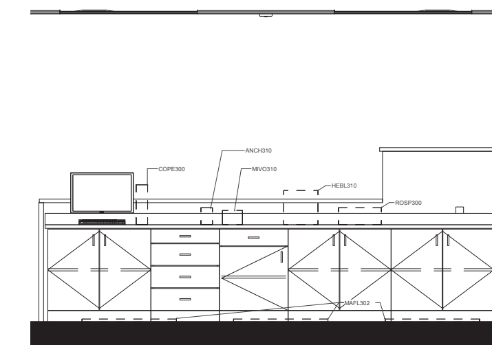
8 LAB Elevation A002-8 1/2" = 1'-0"
