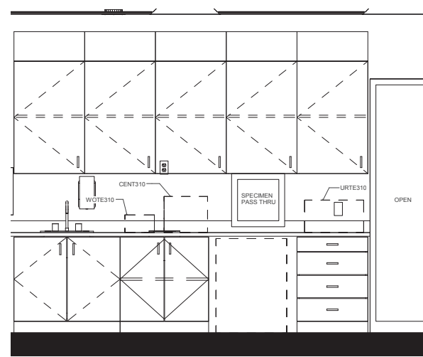
5 LAB Elevation A002-5 1/2" = 1'-0"
