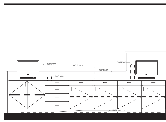
6 LAB Elevation A002-6 1/2" = 1'-0"
