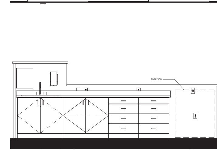
7 LAB Elevation A002-7 1/2" = 1'-0"
