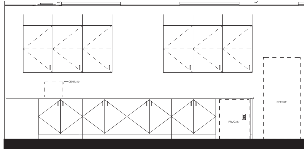
2 LAB Elevation A002-2 1/2" = 1'-0"
