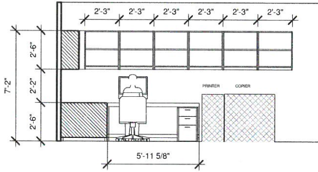
① OUTGOING MAIL- EAST 1/4" = 1'-0"
