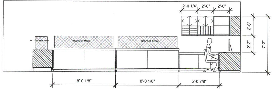
② OUTGOING MAIL- NORTH 1/4" = 1'-0"
