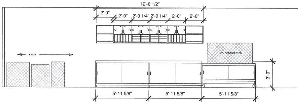
① INCOMING MAIL- SOUTH 1/4" = 1'-0"
