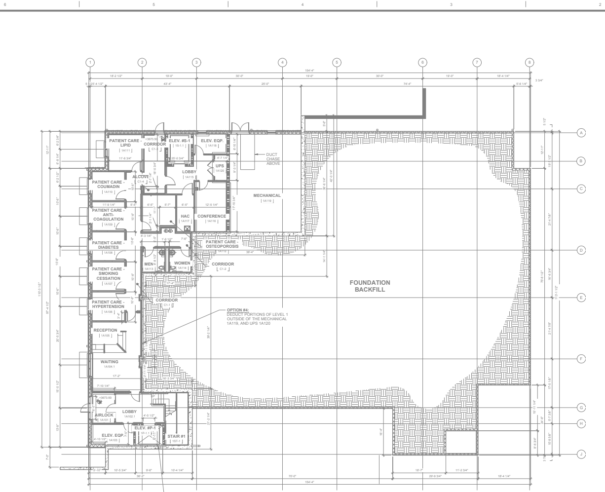
1 LEVEL 1 - DIMENSION PLAN 1/8" = 1'-0" NOTE: SEE BID OPTION #4 & #5 ON AE101.1
