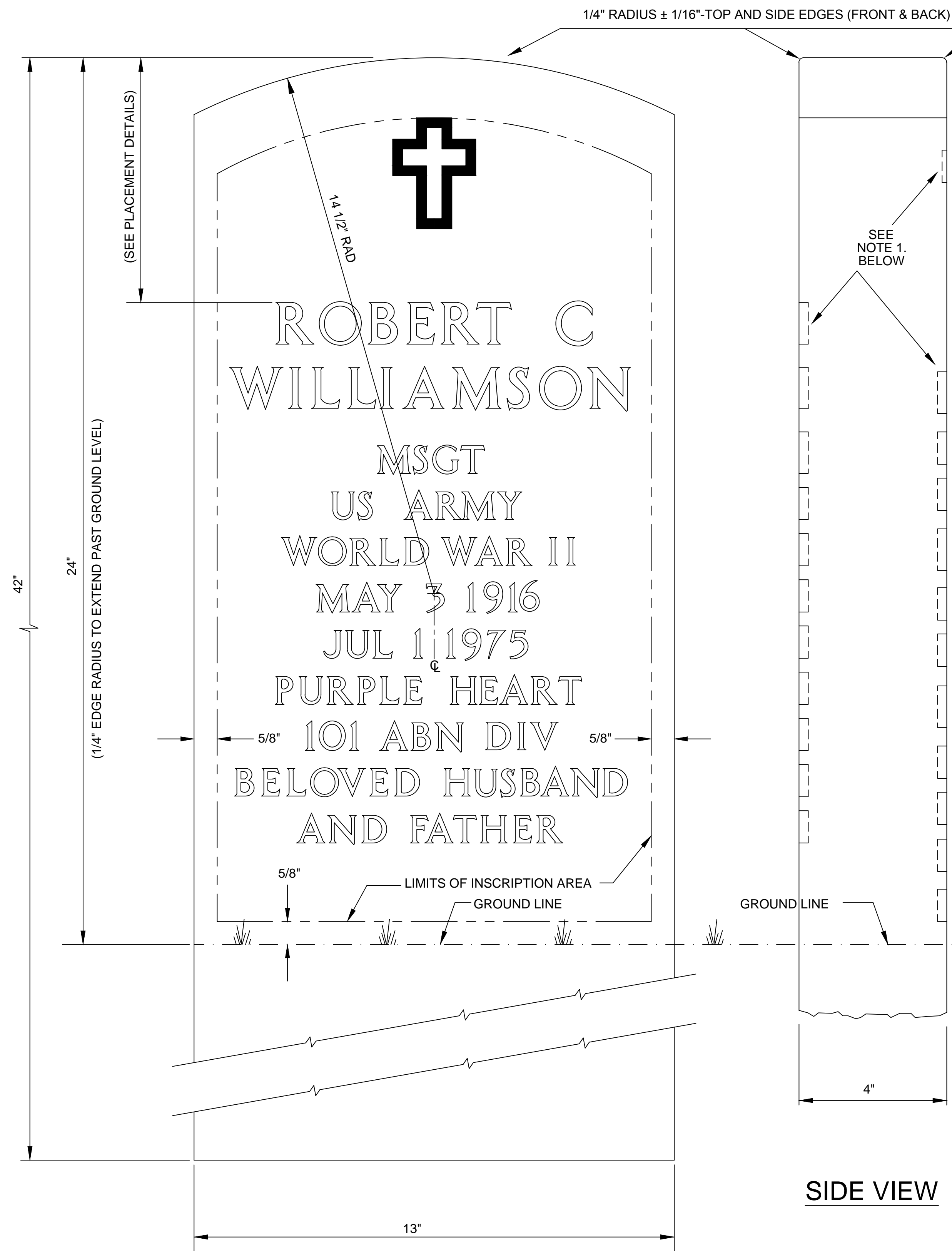
TYPICAL FRONT FACE OF STONE SCALE: 1/2"=1"
