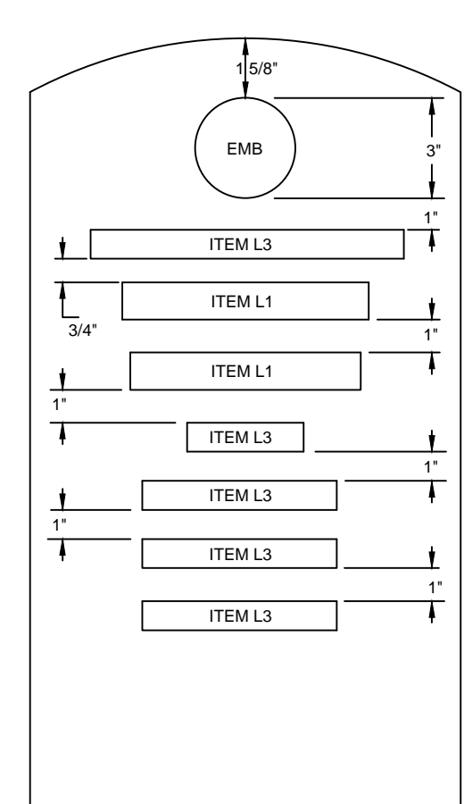
7 LINE INSCRIPTION PLACEMENT AND DETAIL
