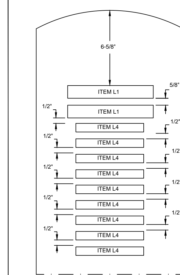
11 LINE INSCRIPTION PLACEMENT AND DETAIL
