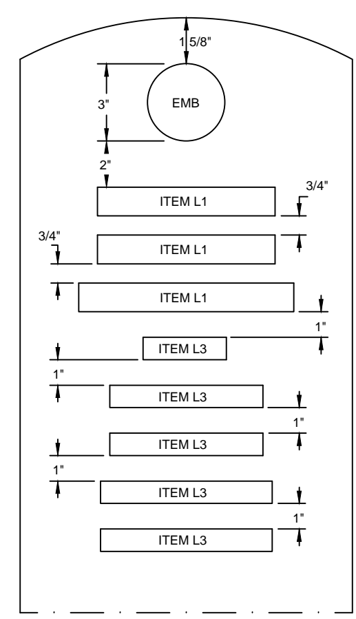
8 LINE INSCRIPTION PLACEMENT AND DETAIL
