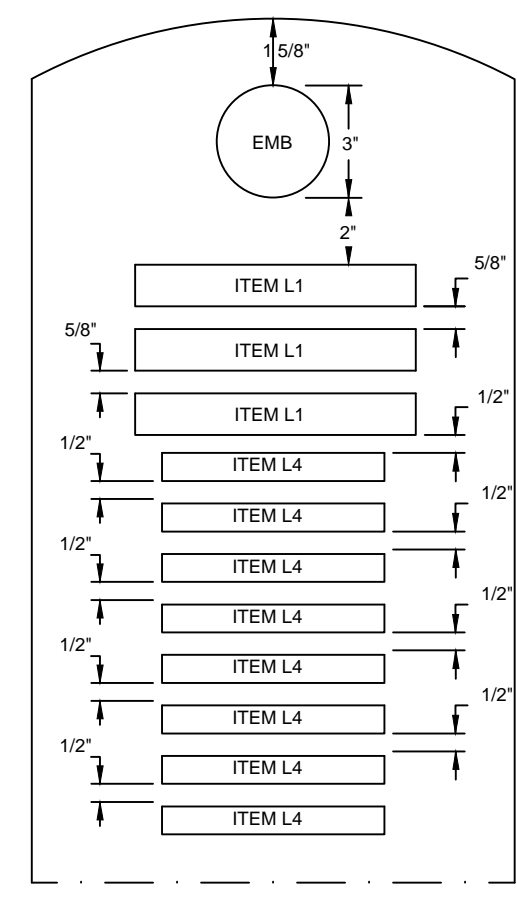
11 LINE INSCRIPTION PLACEMENT AND DETAIL
