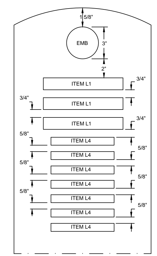
10 LINE INSCRIPTION PLACEMENT AND DETAIL
