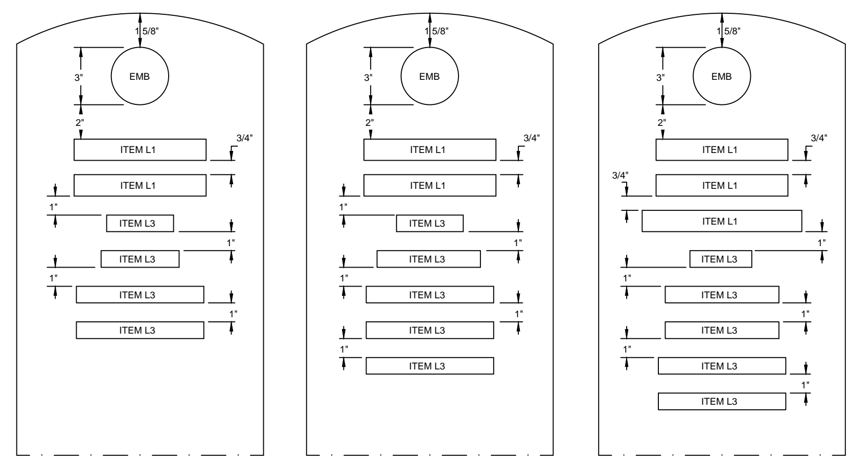
6 LINE INSCRIPTION PLACEMENT AND DETAIL
