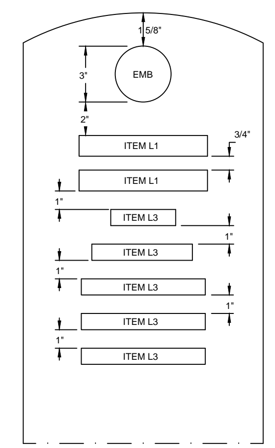
7 LINE INSCRIPTION PLACEMENT AND DETAIL
