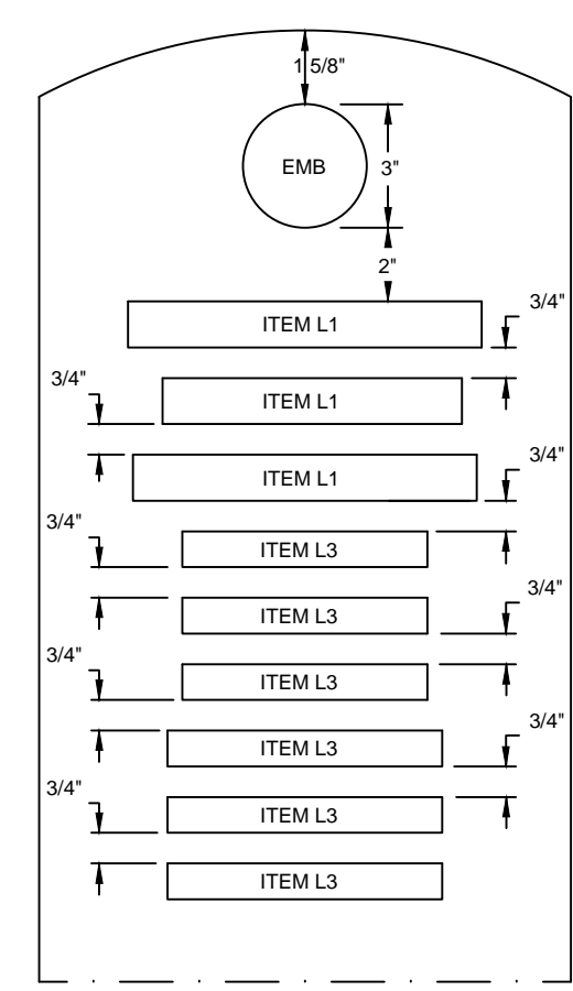
9 LINE INSCRIPTION PLACEMENT AND DETAIL
