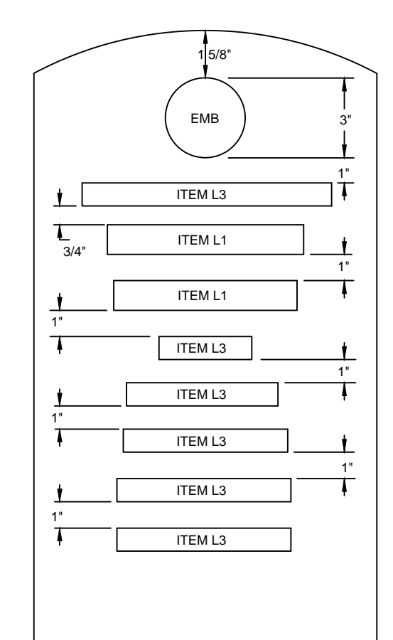
8 LINE INSCRIPTION PLACEMENT AND DETAIL
