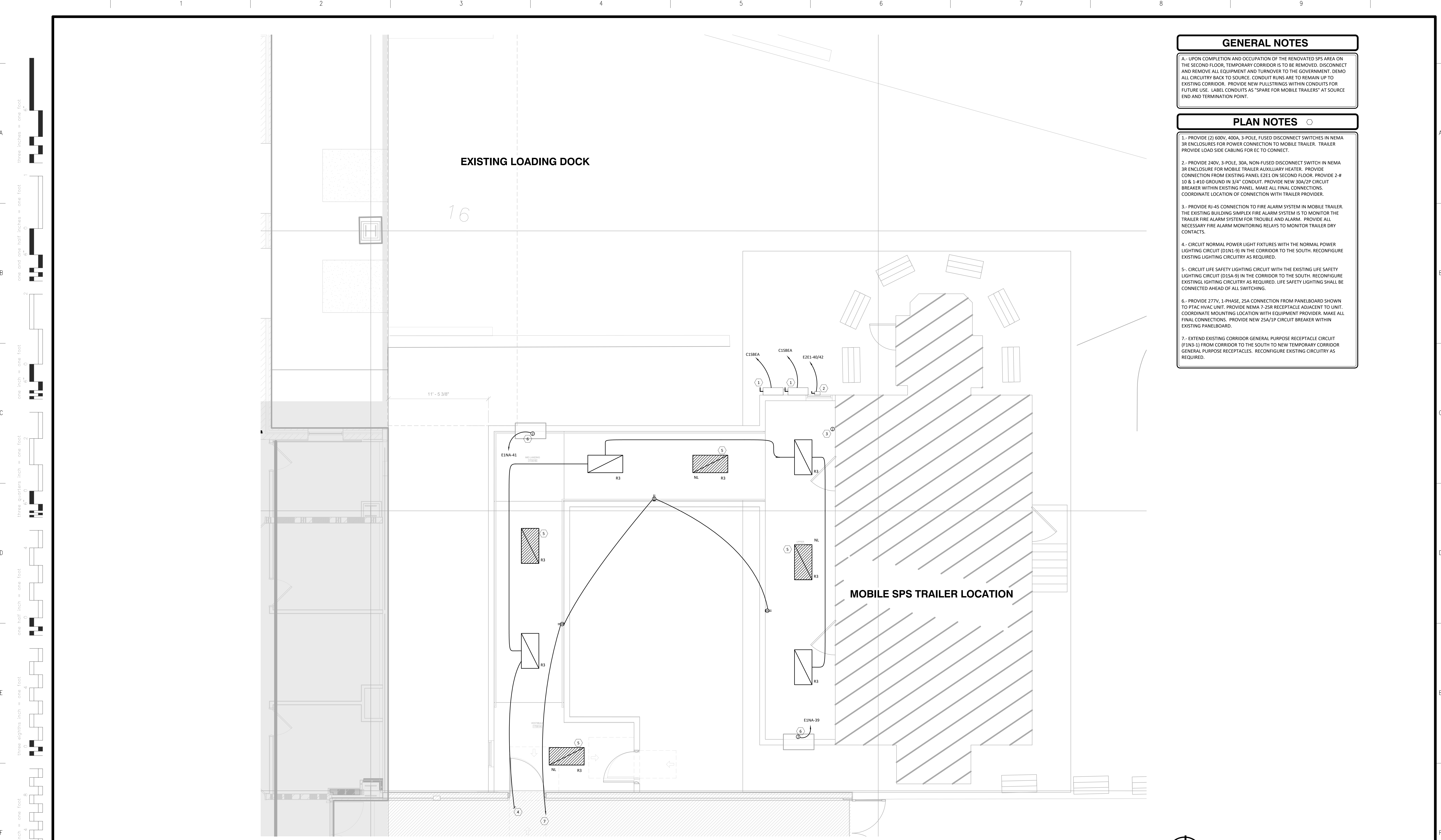
1 ELECTRICAL MOBILE SPS PLAN 1/4" = 1'-0"
