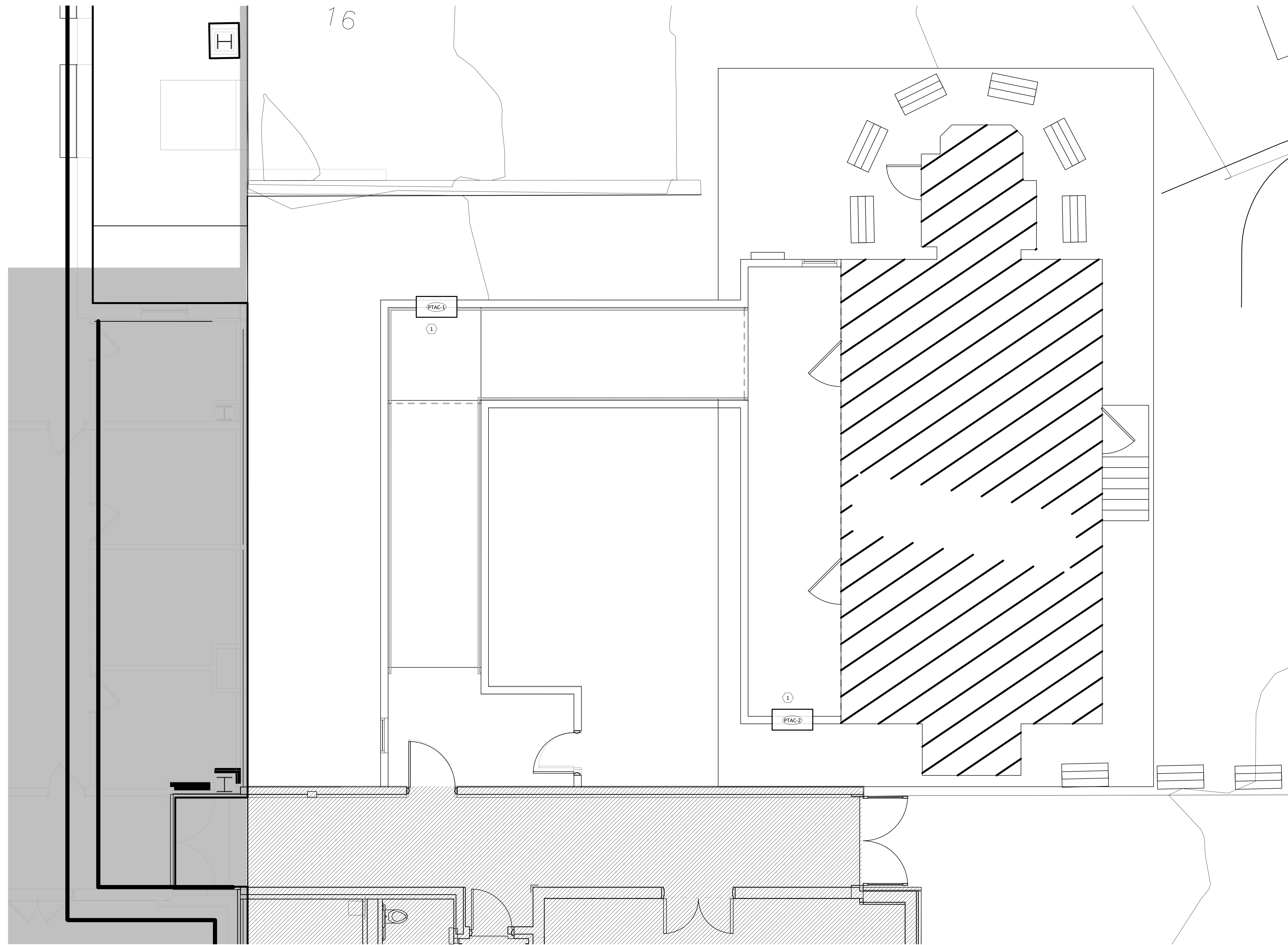
HVAC SITE PLAN SCALE: 1/4" = 1'-0"
