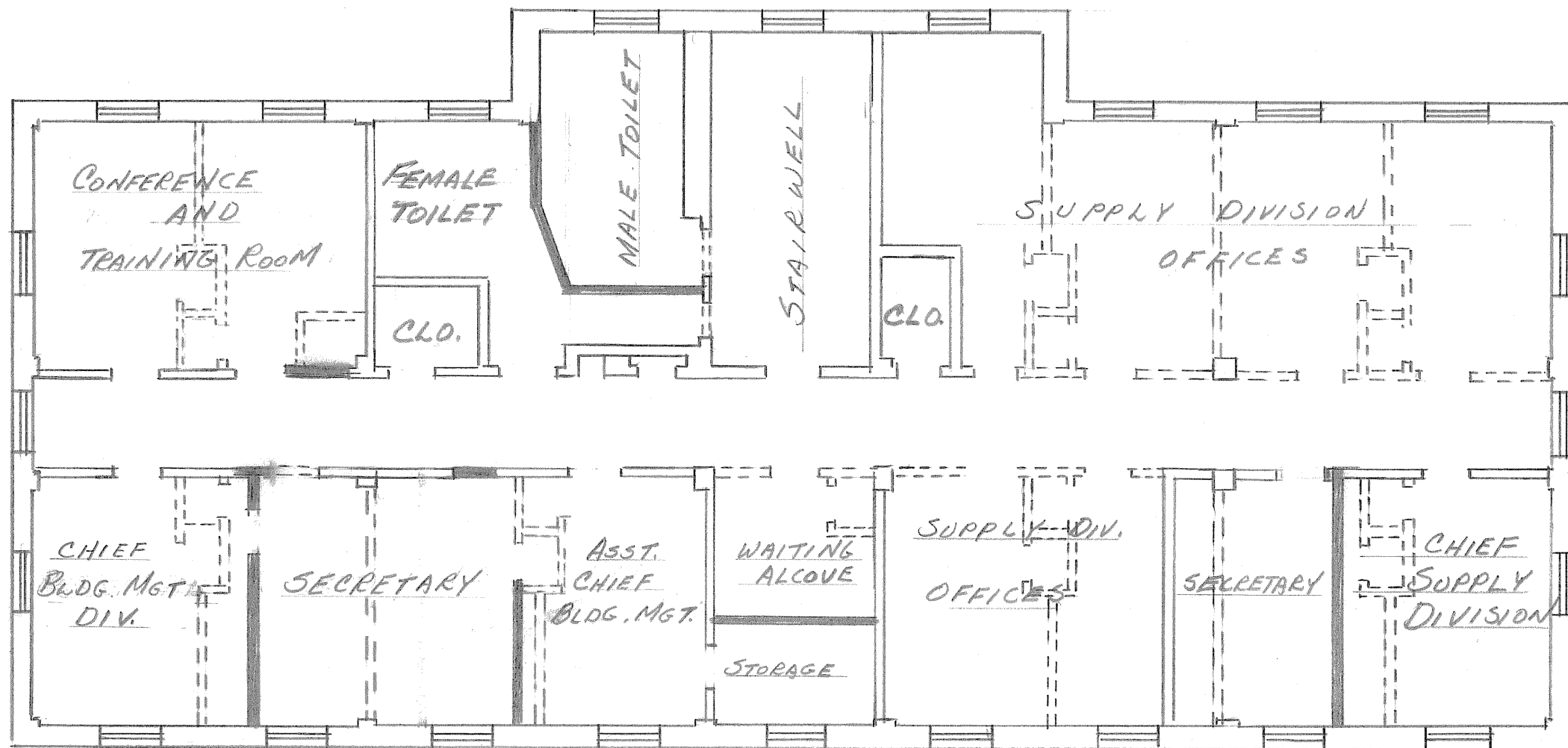
SECOND FLOOR PLAN BLDG. #27 SCALE 1/8" = 1'-0"
