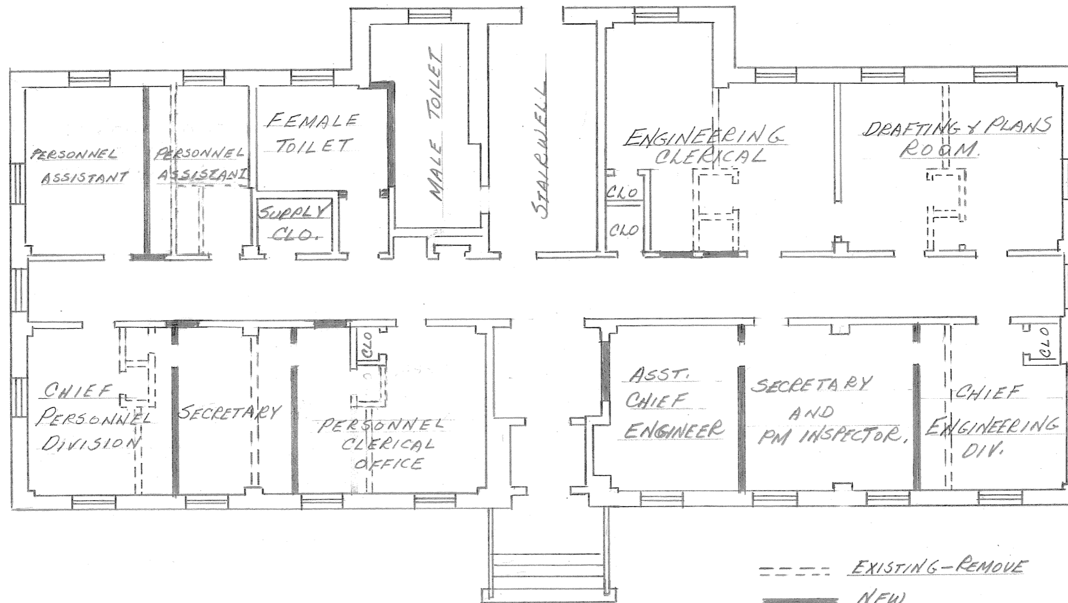
FIRST FLOOR PLAN BLDG No 27 SCALE 1/8" = 1'-0"
