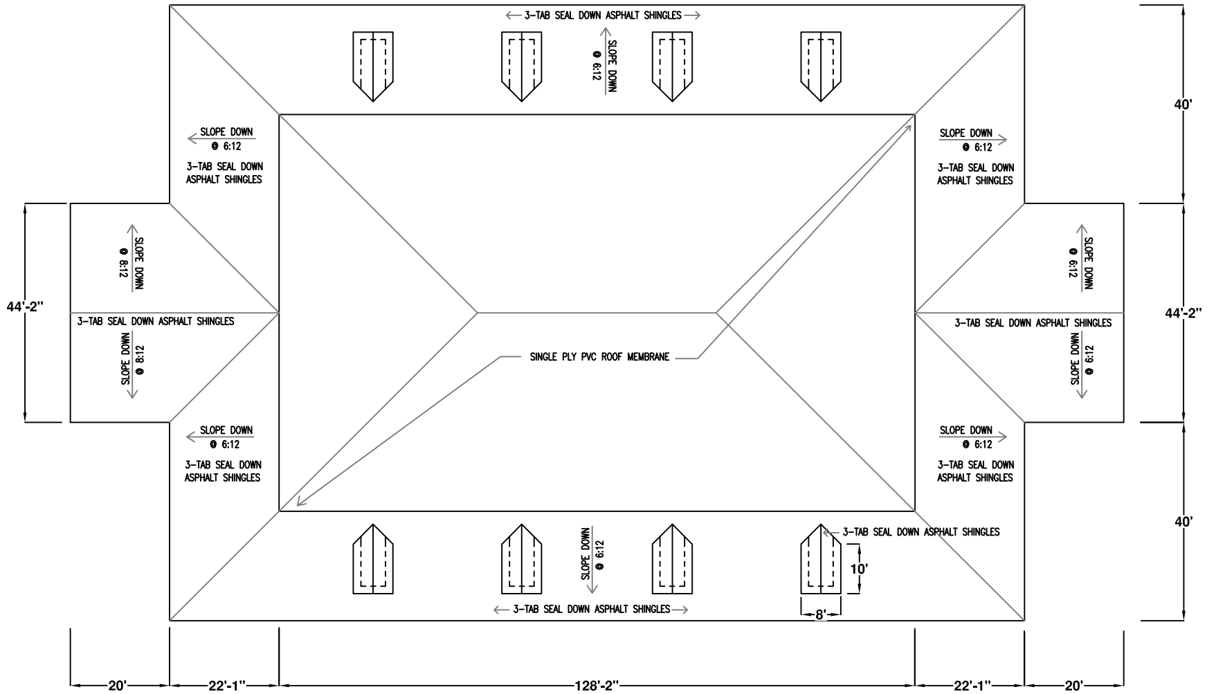
ROOF PLAN
