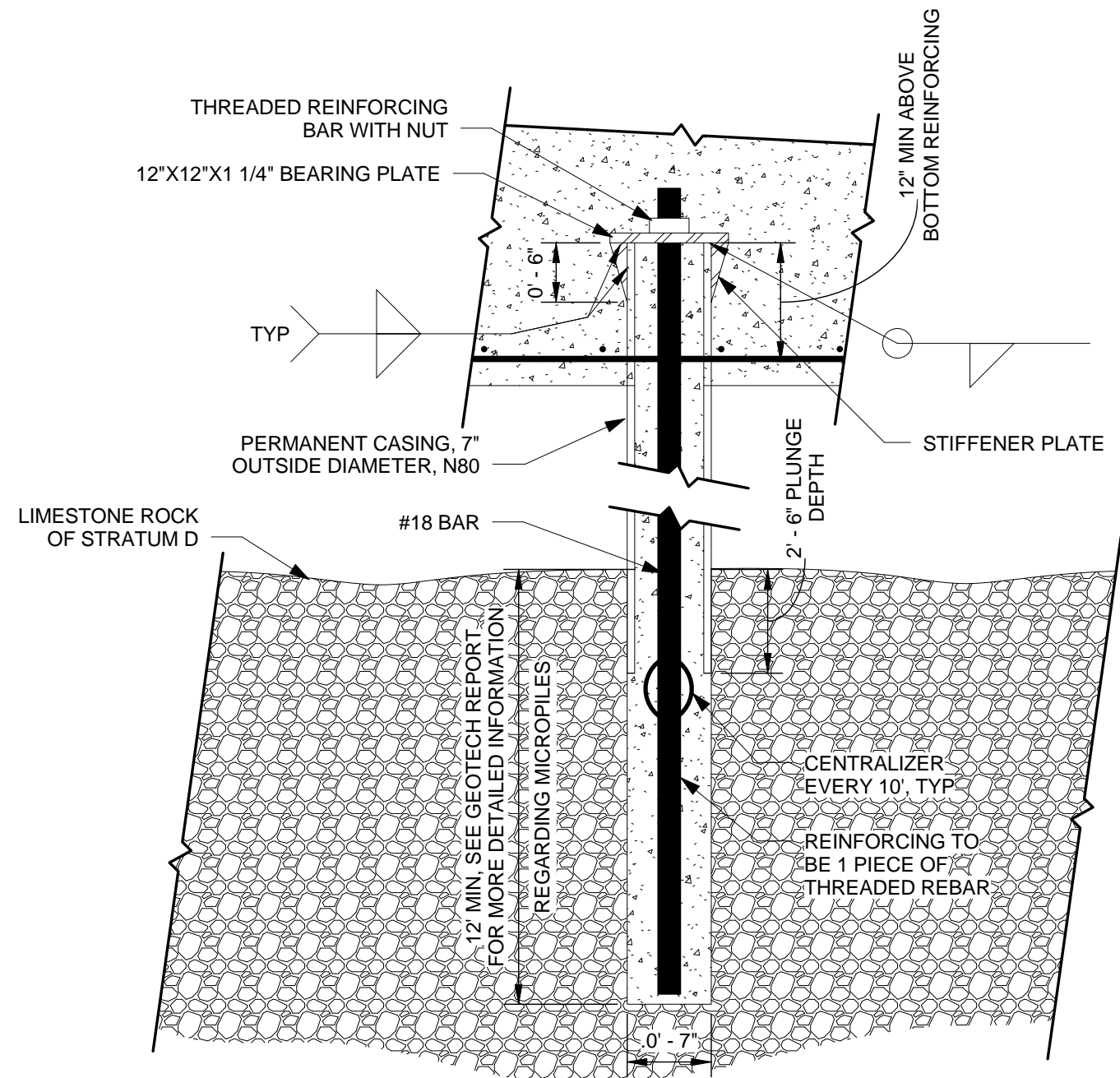
1 Typical Micropile Detail Not to Scale
