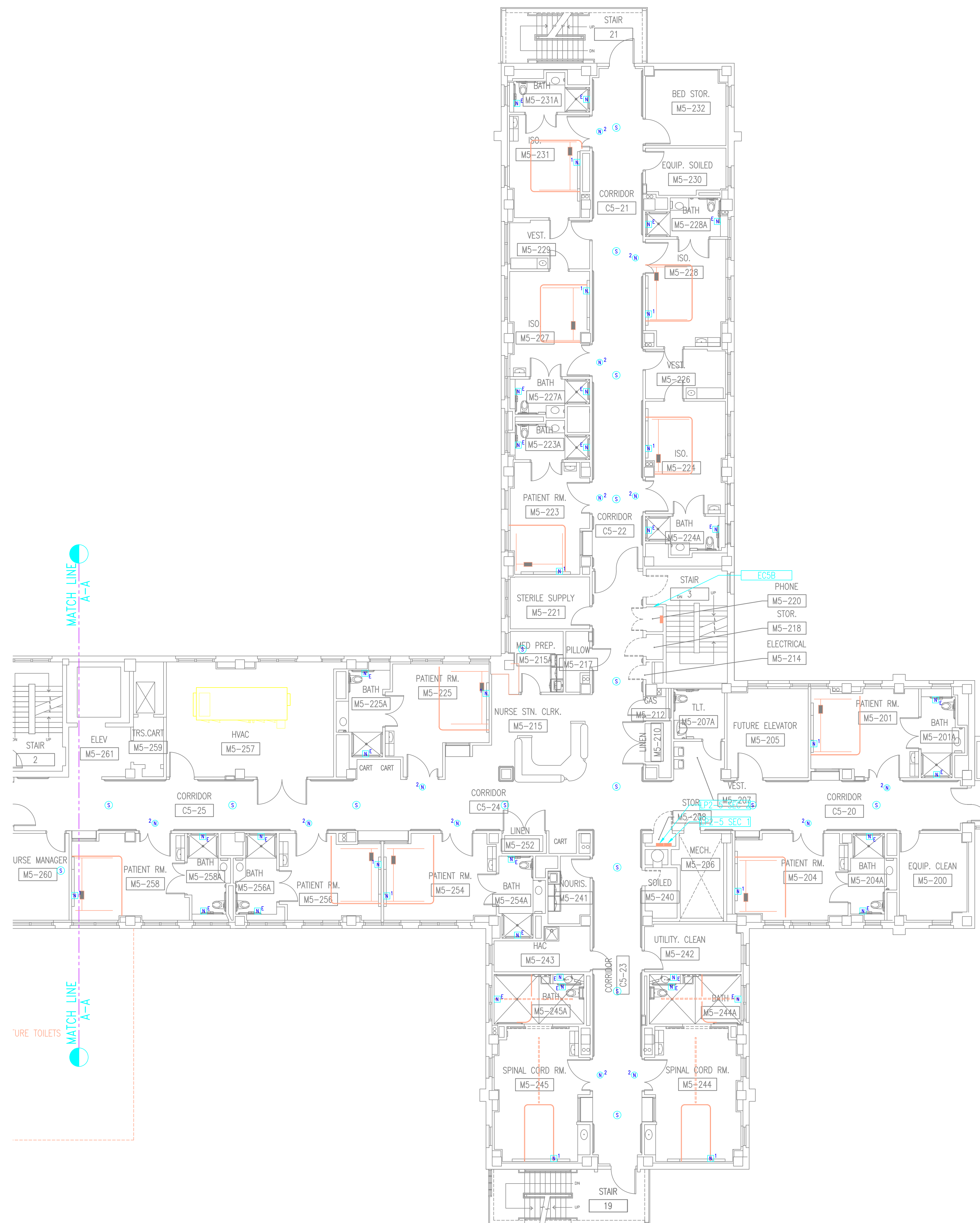
1 PARTIAL FIFTH FLOOR PLAN - INTERCOM/NURSE CALL SCALE: 1/8"=1'-0" NORTH
